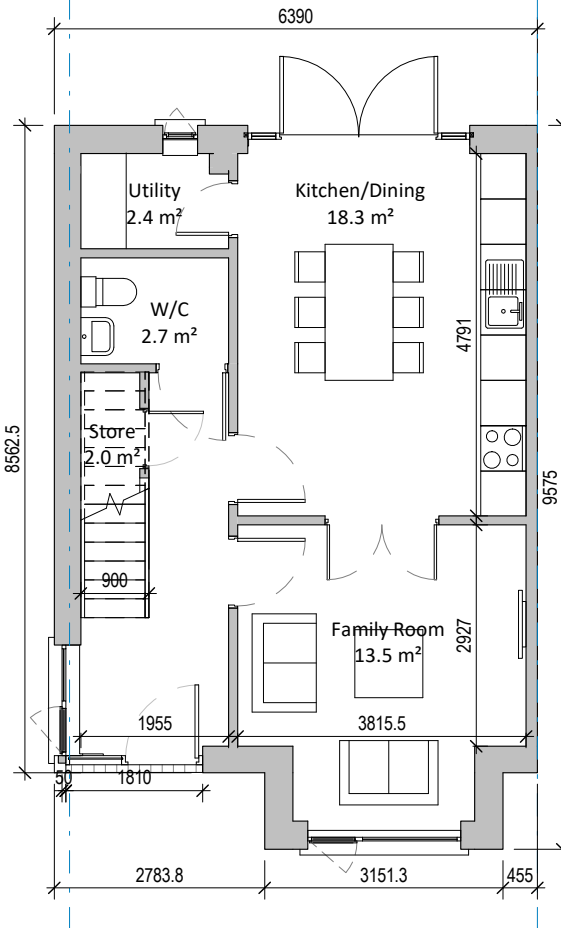
② H08L Level 00 1 : 100
