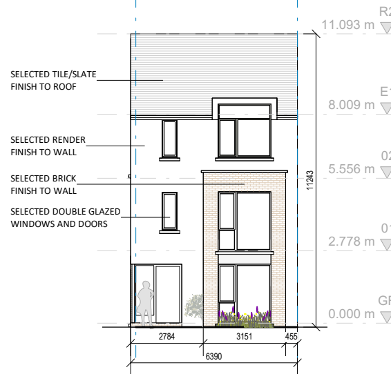
⑥ H08L Render Front Elevation 1 : 200
